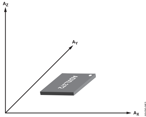
Figure 52. Axes of Acceleration Sensitivity (Corresponding Output Increases When Accelerated Along the Sensitive Axis)
