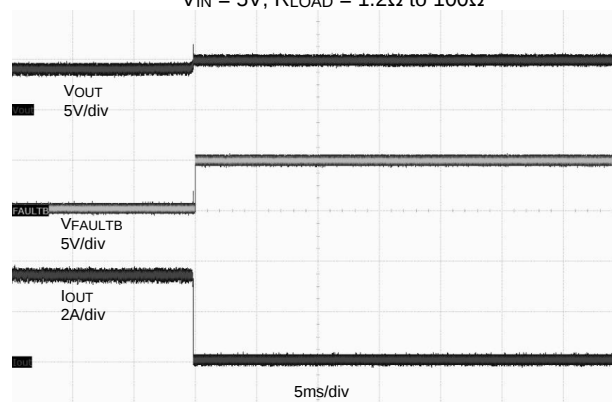
Overcurrent Recovery V_{IN} = 5\text{V} , R_{LOAD} = 1.2\Omega to 100\Omega
