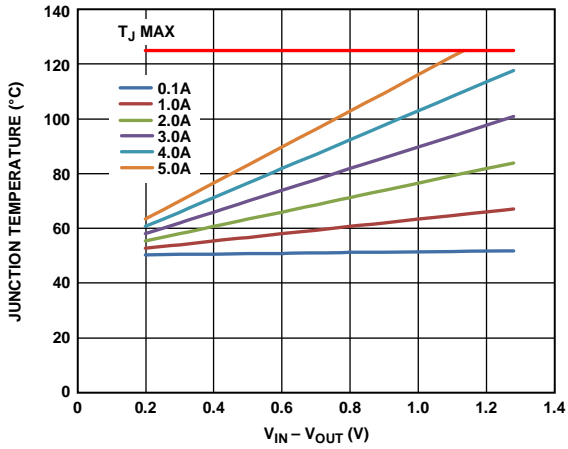
Figure 53. 1000 mm 2 of PCB Copper, T_B = 50^\circ\text{C}
