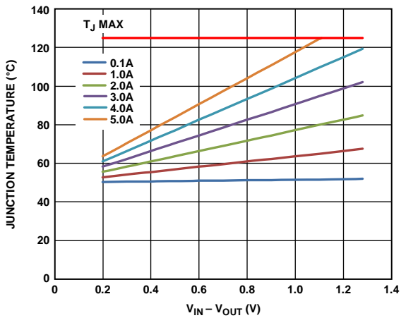
Figure 54. 500 mm 2 of PCB Copper, T_B = 50^\circ\text{C}
